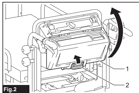
Fig. 2 ► 1. Cover 2. Lock lever
